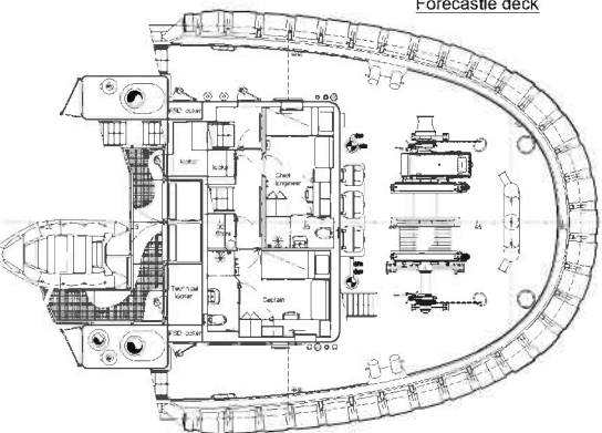
Forecastle deck
