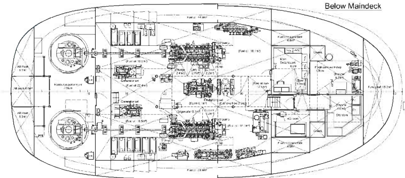
Below Maindeck
