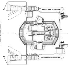
Bridge deck
