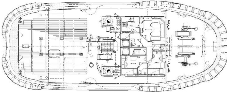
Main deck
